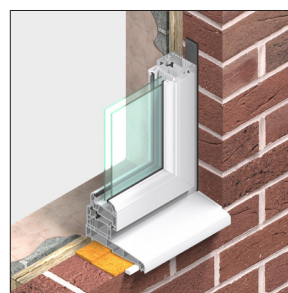
Fig. 4 TP650 installed (FM330 under sill)
